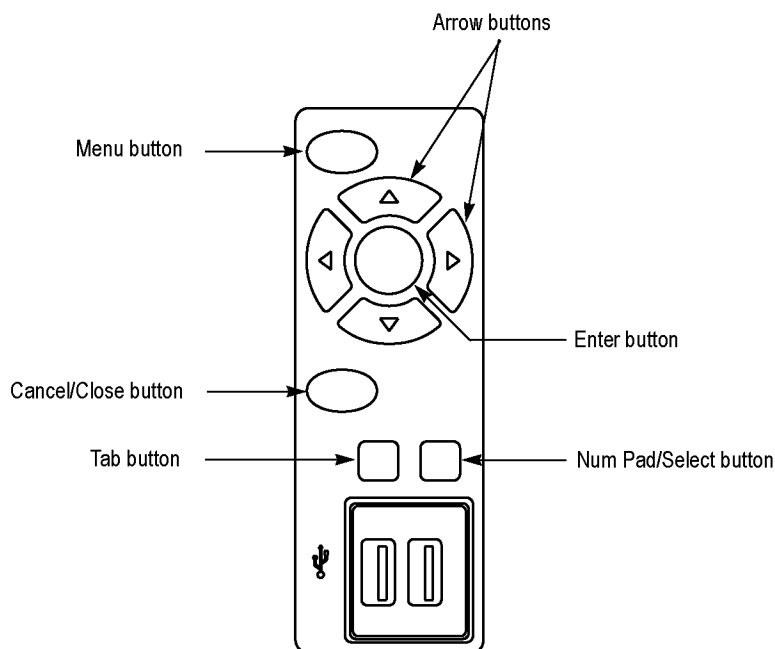
Figure 2-8: Front panel showing the menu controls
